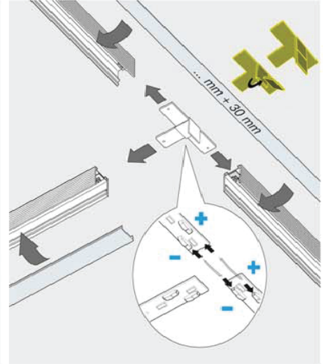
T Junction trimless D8-6340
