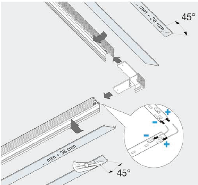
90° wall to wall / ceiling to ceiling Junction D8-6339
