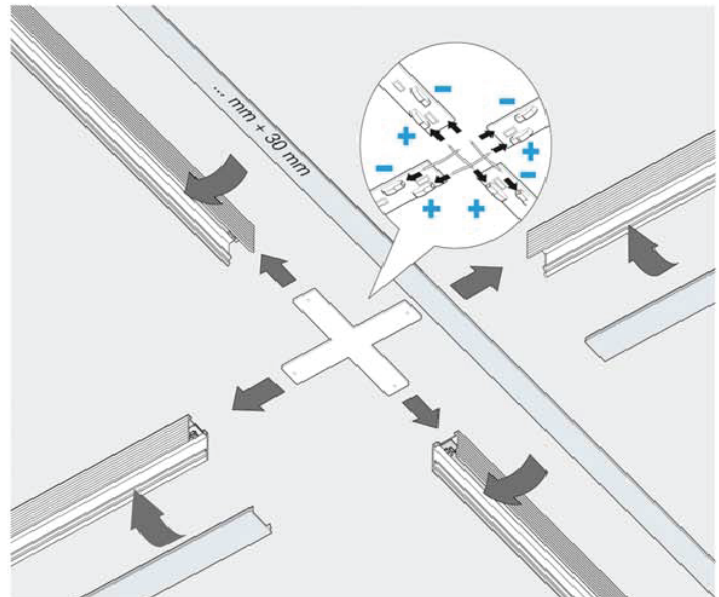
X Junction trimless D8-6341
