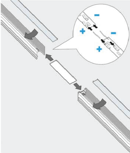
Linear Junction D8-6338
