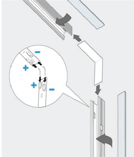
90° wall to ceiling Junction D8-6337
