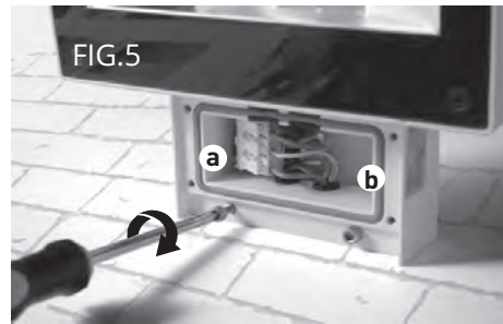
SOLARIS Wire connection.
