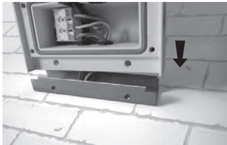
Fix the plate to the wall.
